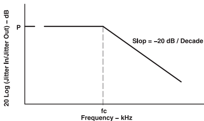
Figure 2. Jitter Transfer
