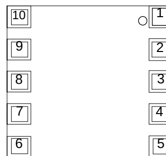
10-Pin Plastic Module Package ; Bottom View
