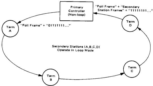
FIGURE 9b — EXAMPLE OF EXTERNAL LOOP LOGIC
