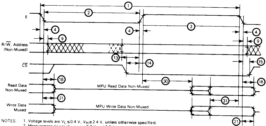
FIGURE 6 — BUS TIMING
