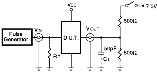
Figure 12. AC Test Load Circuit
