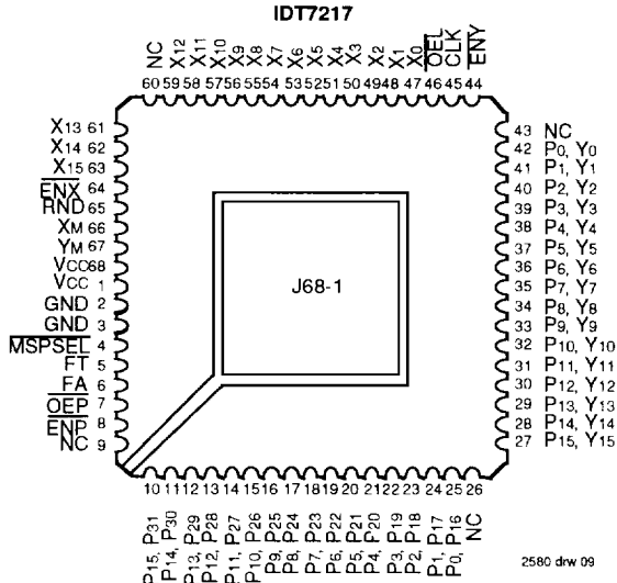
PLCC TOP VIEW
