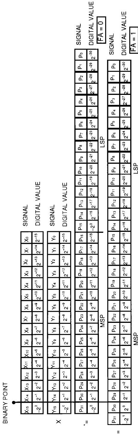
Figure 6. Fractional Two's Complement Notation
