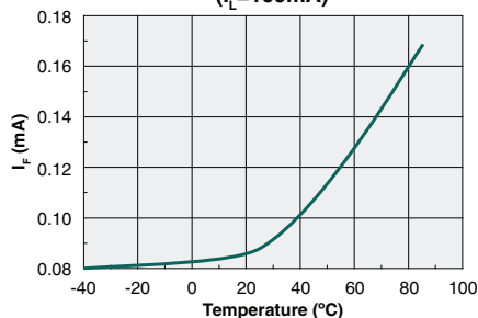
Typical I_F to Operate vs. Temperature ( I_L=100\text{mA} )
