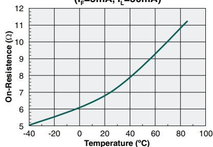
Typical On-Resistance vs. Temperature ( I_F=5\text{mA} , I_L=50\text{mA} )
