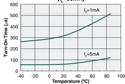
Typical Turn-On Time vs. Temperature ( I_L=50\text{mA} )
