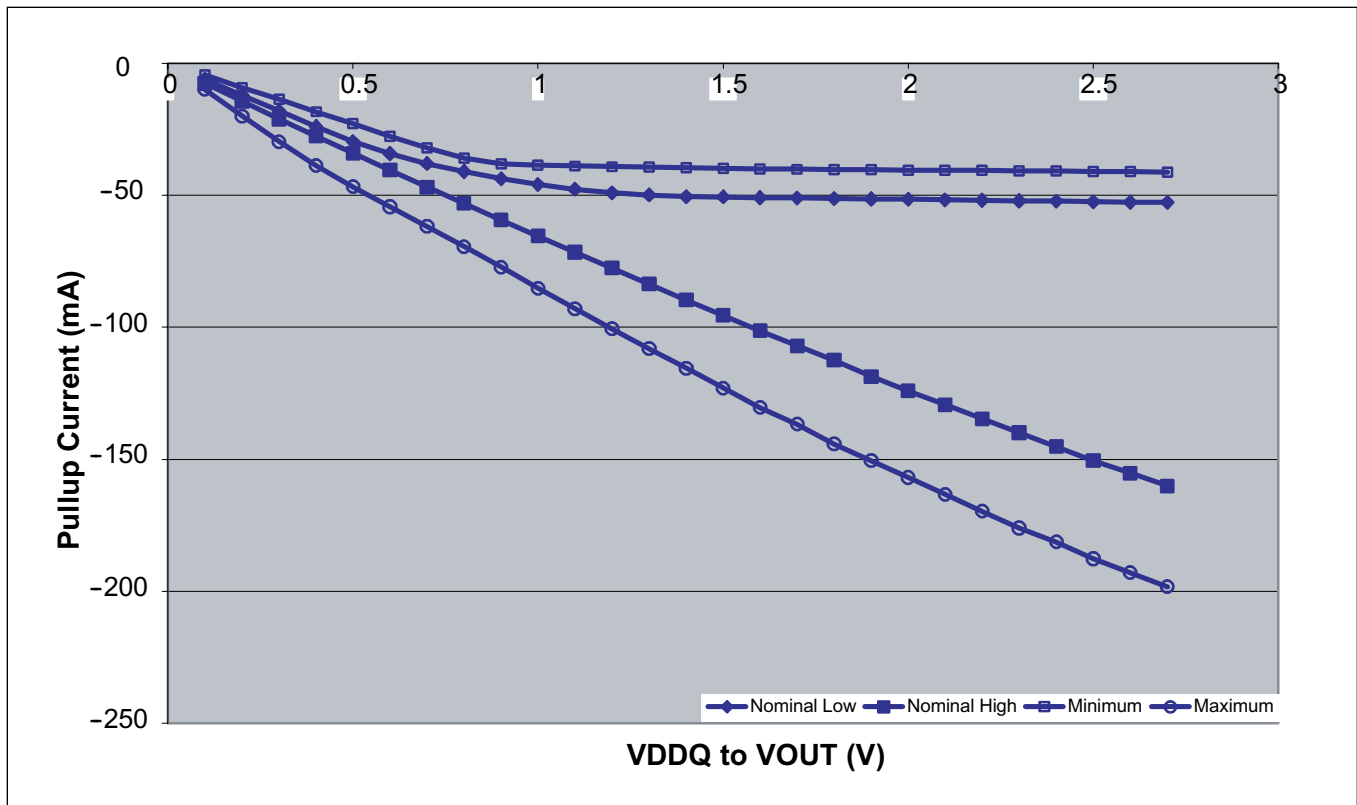
Pullup characteristics for Full Strength Output Driver
