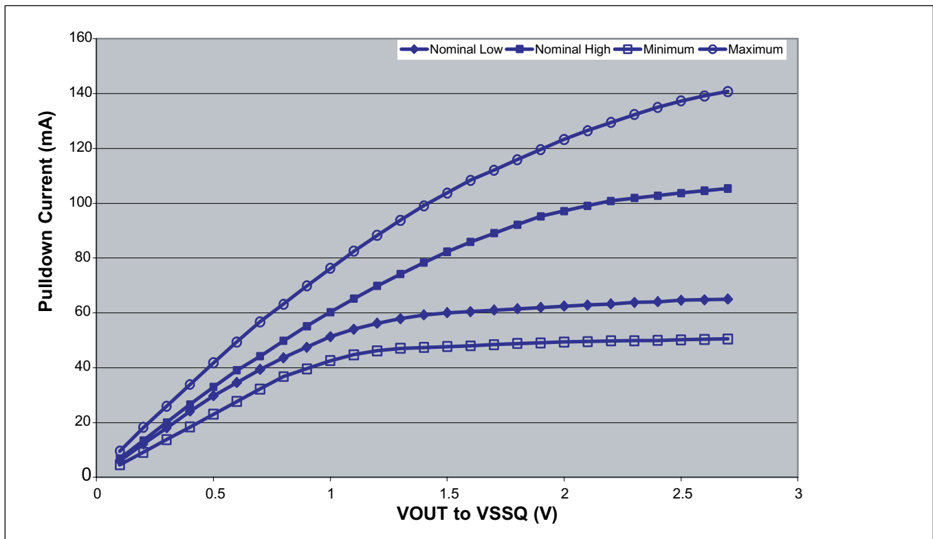
Pulldown characteristics for Full Strength Output Driver
