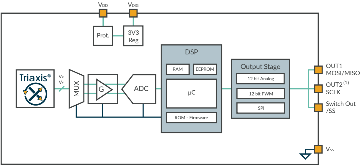
Figure 1 – Block Diagram
