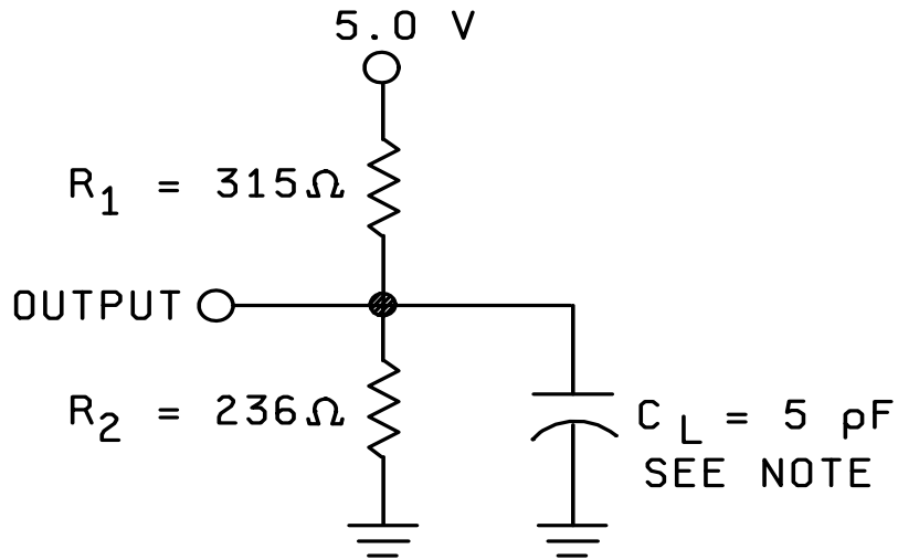
CIRCUIT A OR EQUIVALENT
