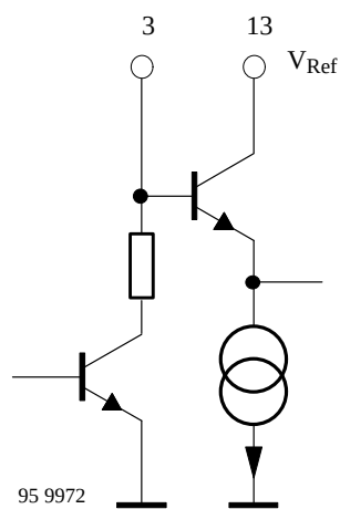
Figure 6. Pin 3 RC_{wake}
