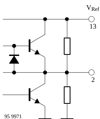
Figure 5. Pin 2 OP_{out}
