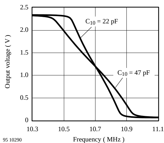
Figure 28. FM-discriminator characteristic
