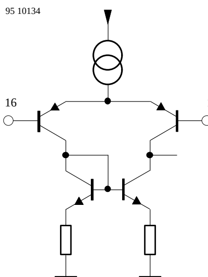
Figure 19. Pin 16 OP_{in-}
