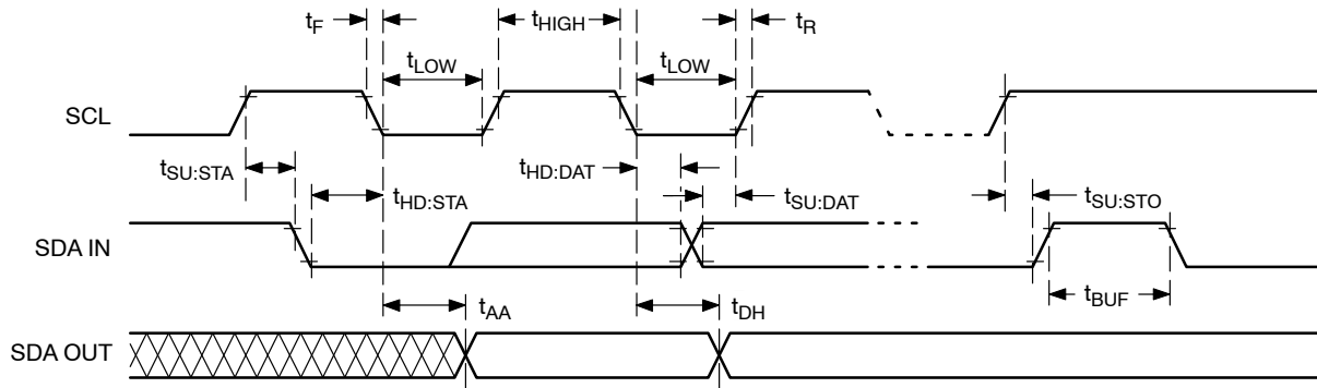
Figure 8. Bus Timing
