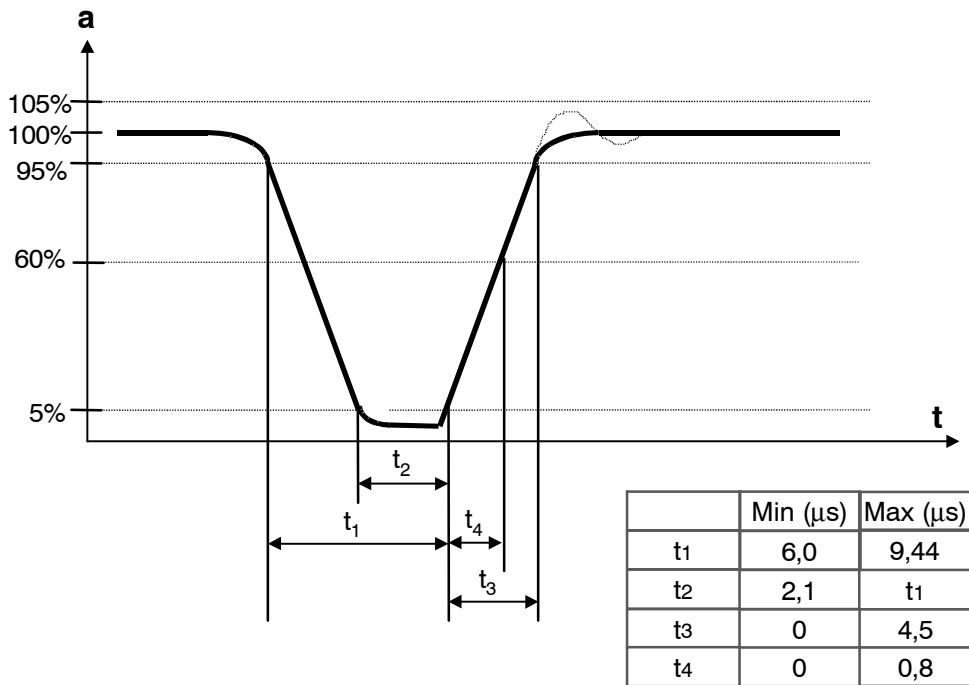
Figure 2. 100% Modulation Waveform
