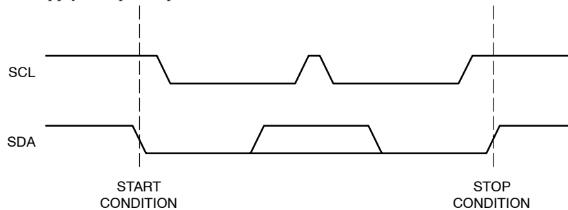
Figure 5. Start/Stop Timing
