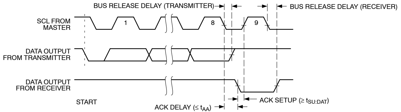
Figure 7. Acknowledge Timing
