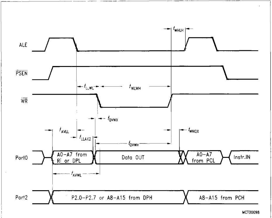
Figure 9 Data Memory Write Cycle
