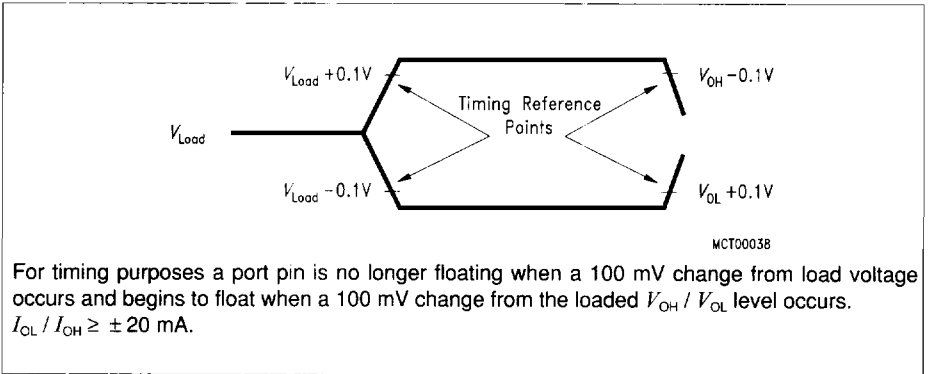
Figure 12 AC Testing: Float Waveforms
