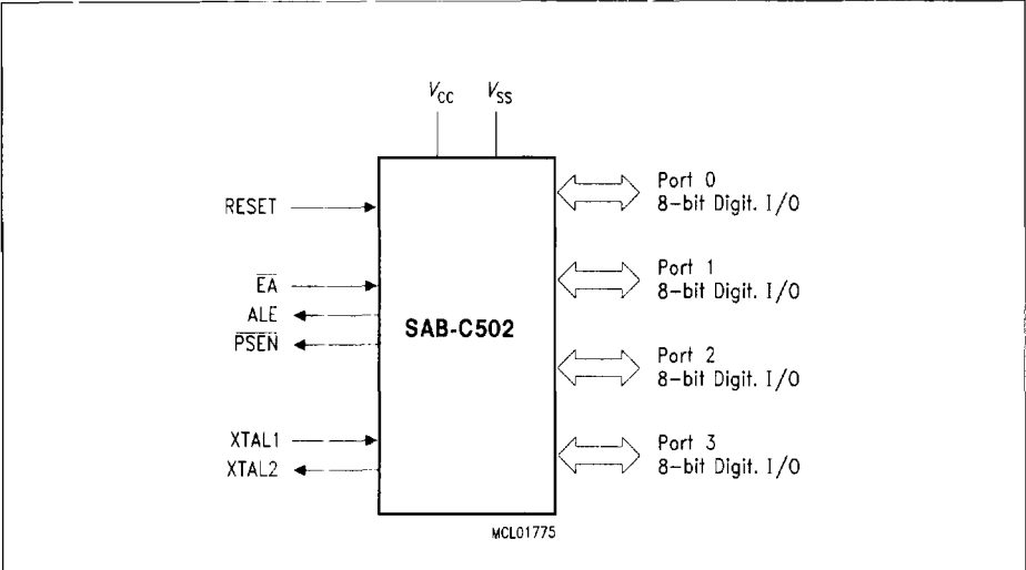
Logic Symbol
