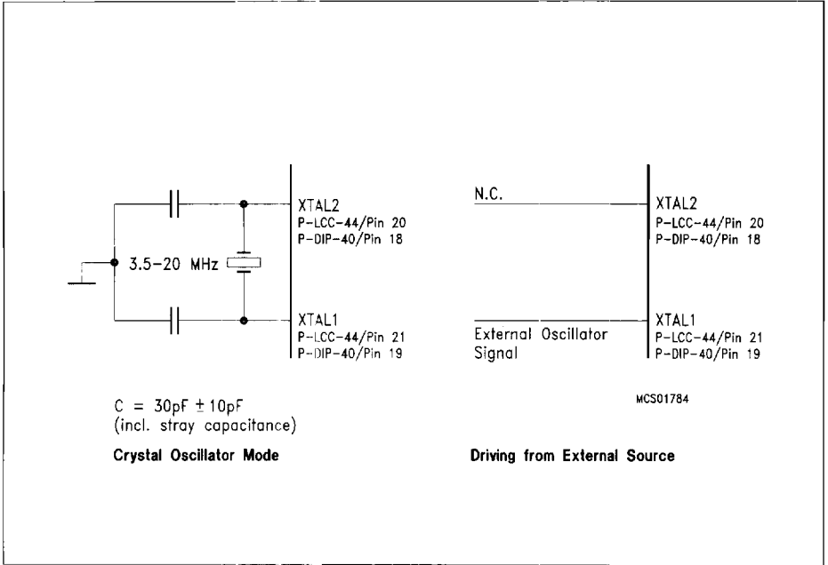
Figure 14 Recommended Oscillator Circuits
