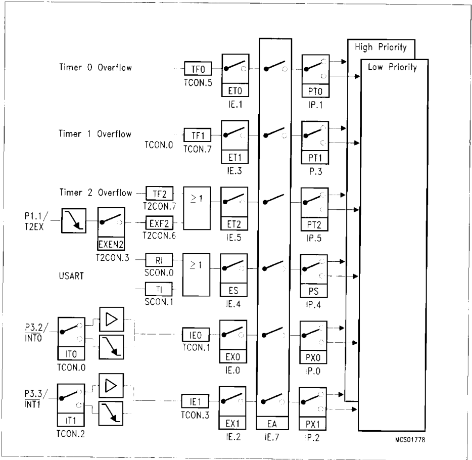
Figure 4 Interrupt Request Sources
