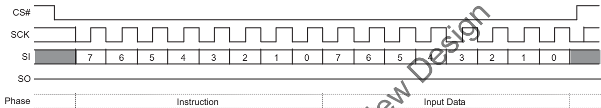
Figure 6. Single Bit Wide Input Command
