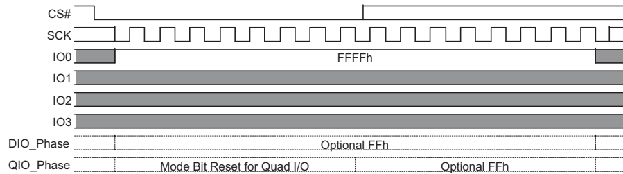
Figure 52. Continuous Read Mode Reset for Fast Read Dual or Quad I/O
