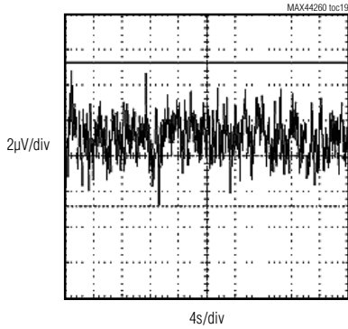
0.1Hz TO 10Hz OUTPUT-VOLTAGE NOISE
