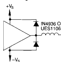
PROTECTION, INDUCTIVE LOAD
