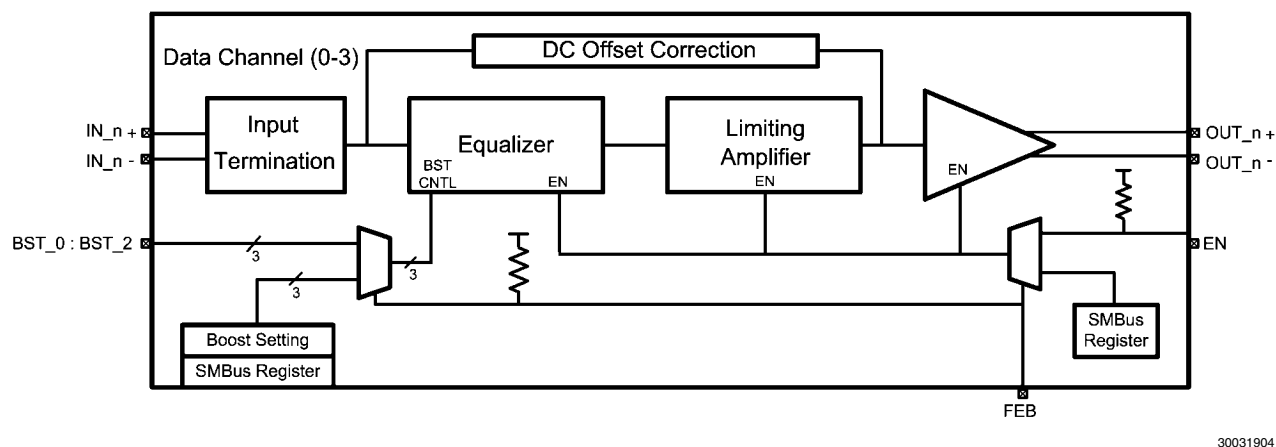
FIGURE 6. Simplified Block Diagram
