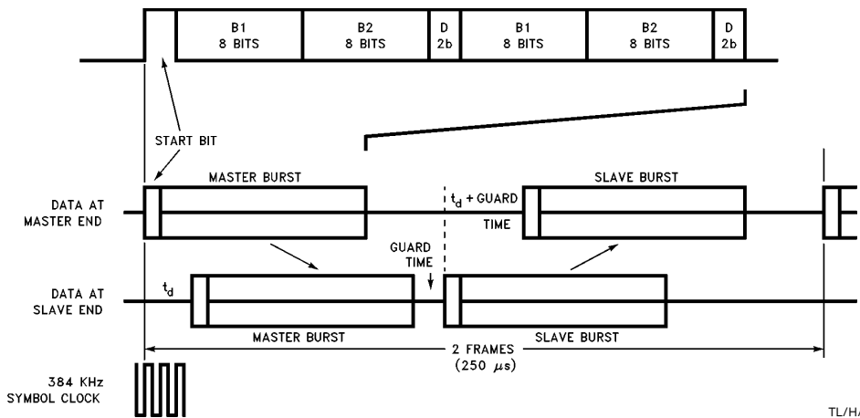
FIGURE 5. Burst Mode Timing on the Line
