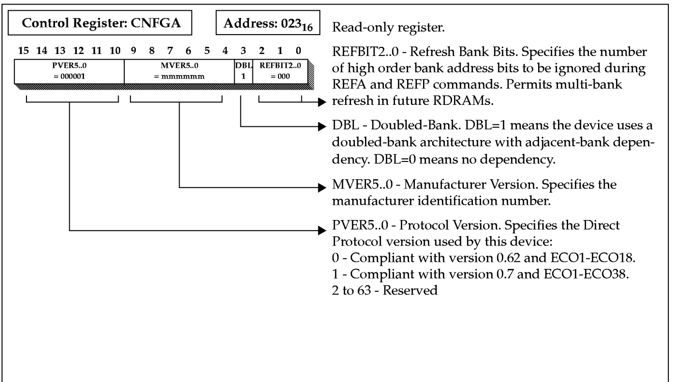
Figure 28: CNFGA Register
