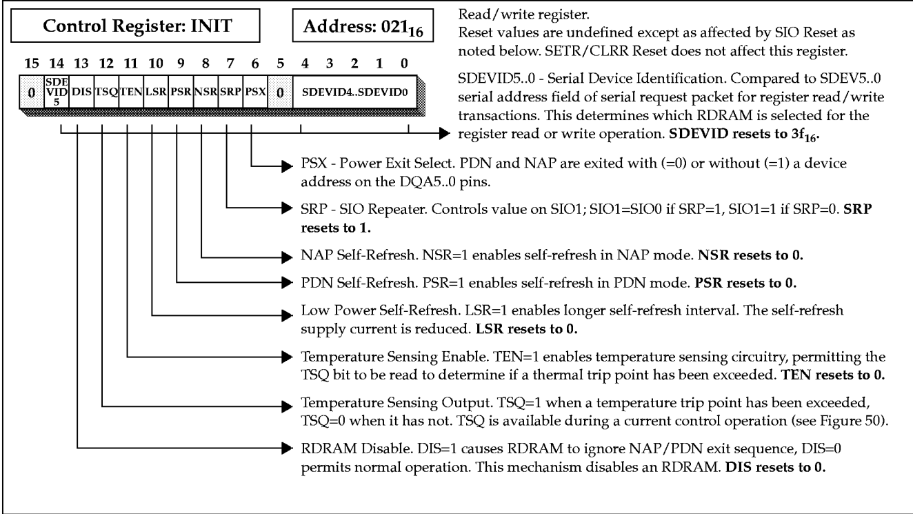
Figure 27: INIT Register
