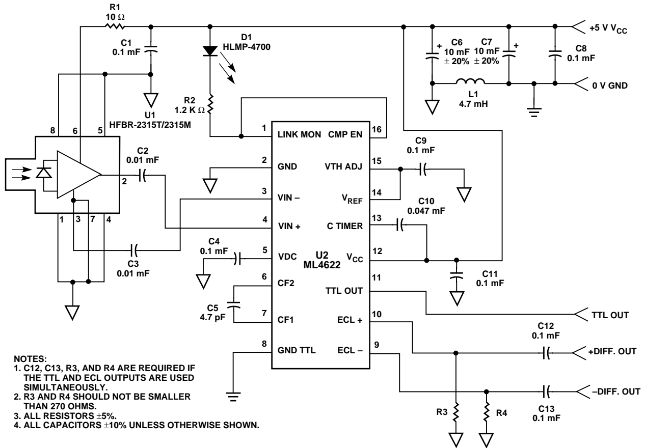
Figure 2. Recommended Receiver Circuit.
