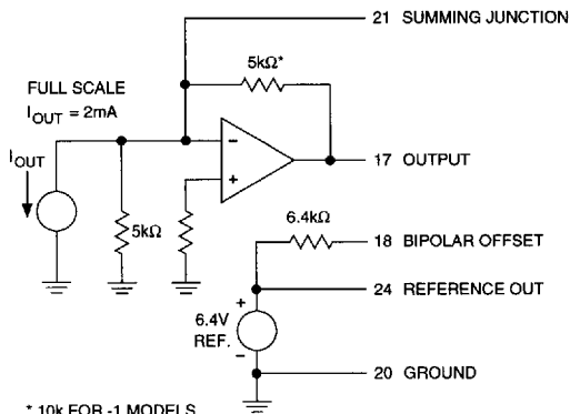
Figure 5. Output Circuit
