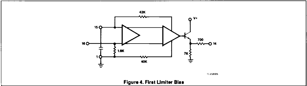
Figure 4. First Limiter Bias
