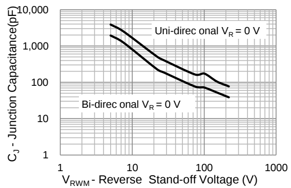
Fig.4 Typical Capacitance
