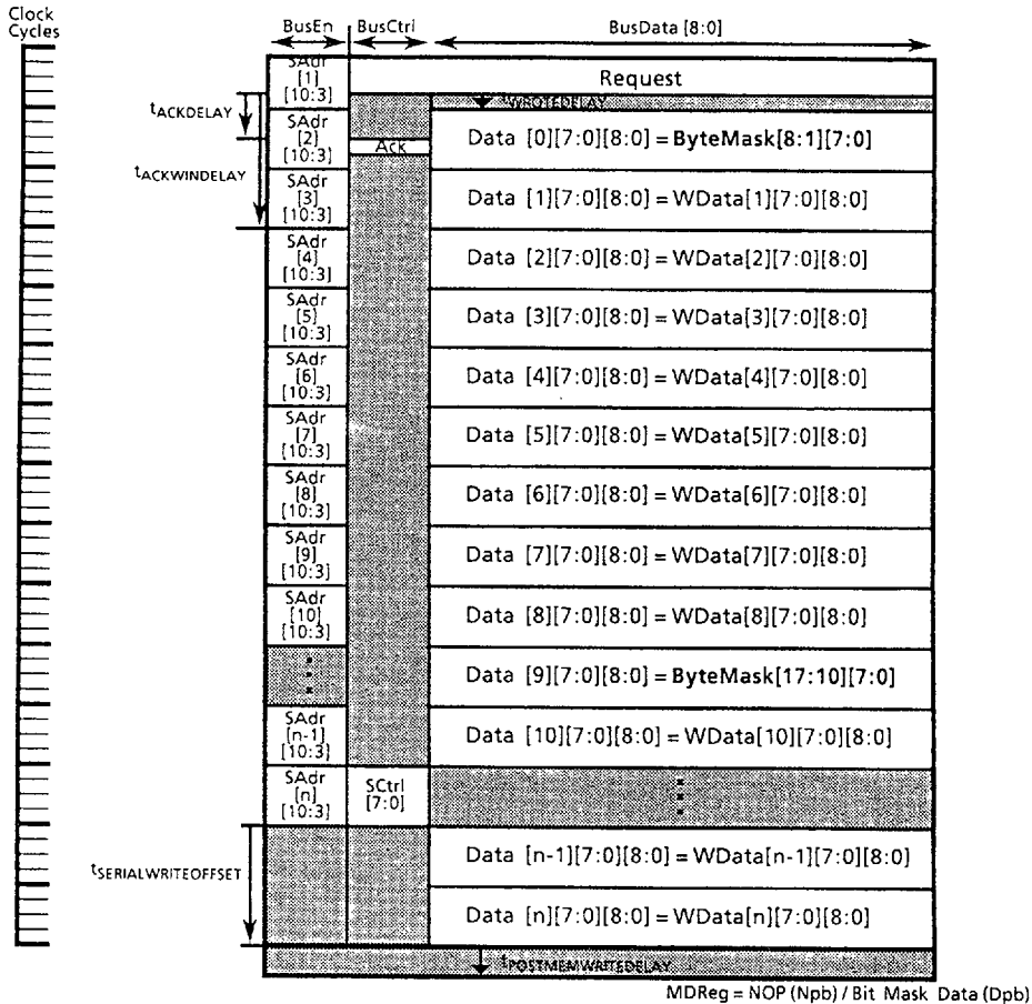
Figure 20. Non-sequential Data Write Transaction with Byte Masking (Npb/Dpb)
