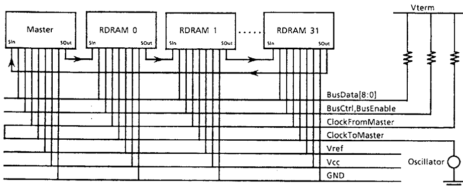
Figure 3. Rambus System
