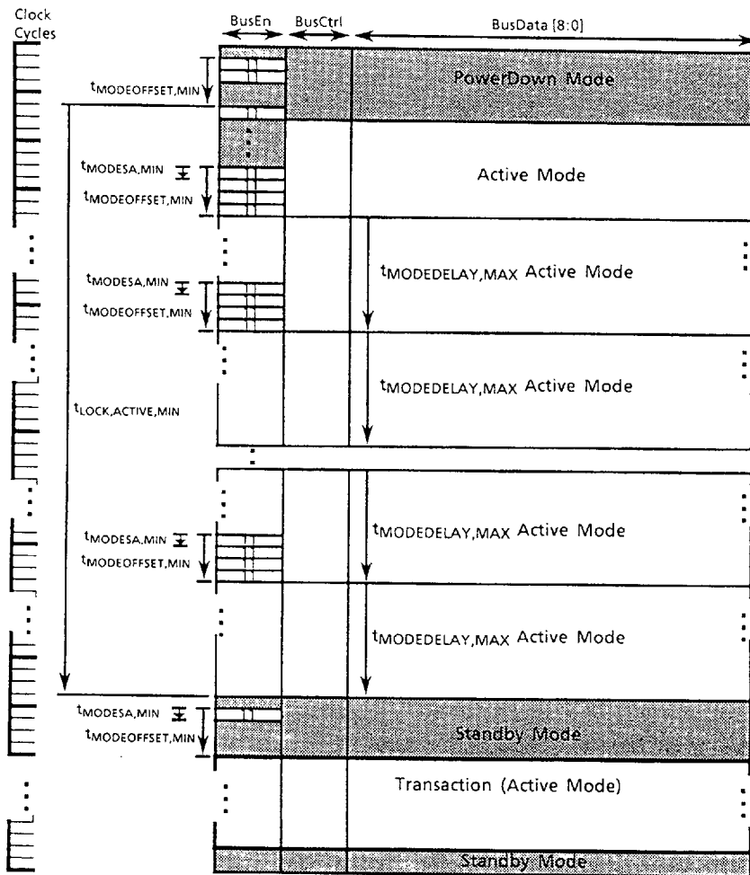
Figure 28. PowerDown Mode to Active Mode Transition
