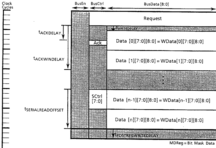
Figure 17. Data-per-bit (Dpb) Write Transactions
