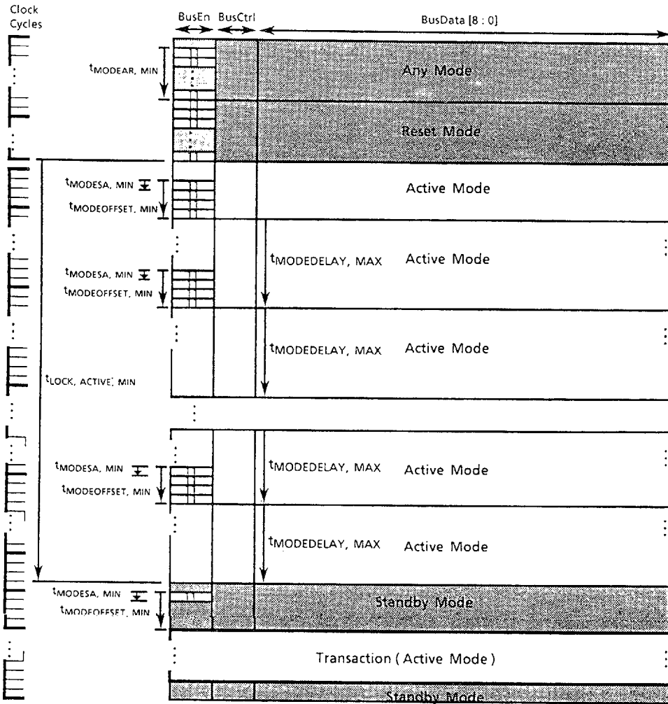
Figure 26. Reset Mode Transition
