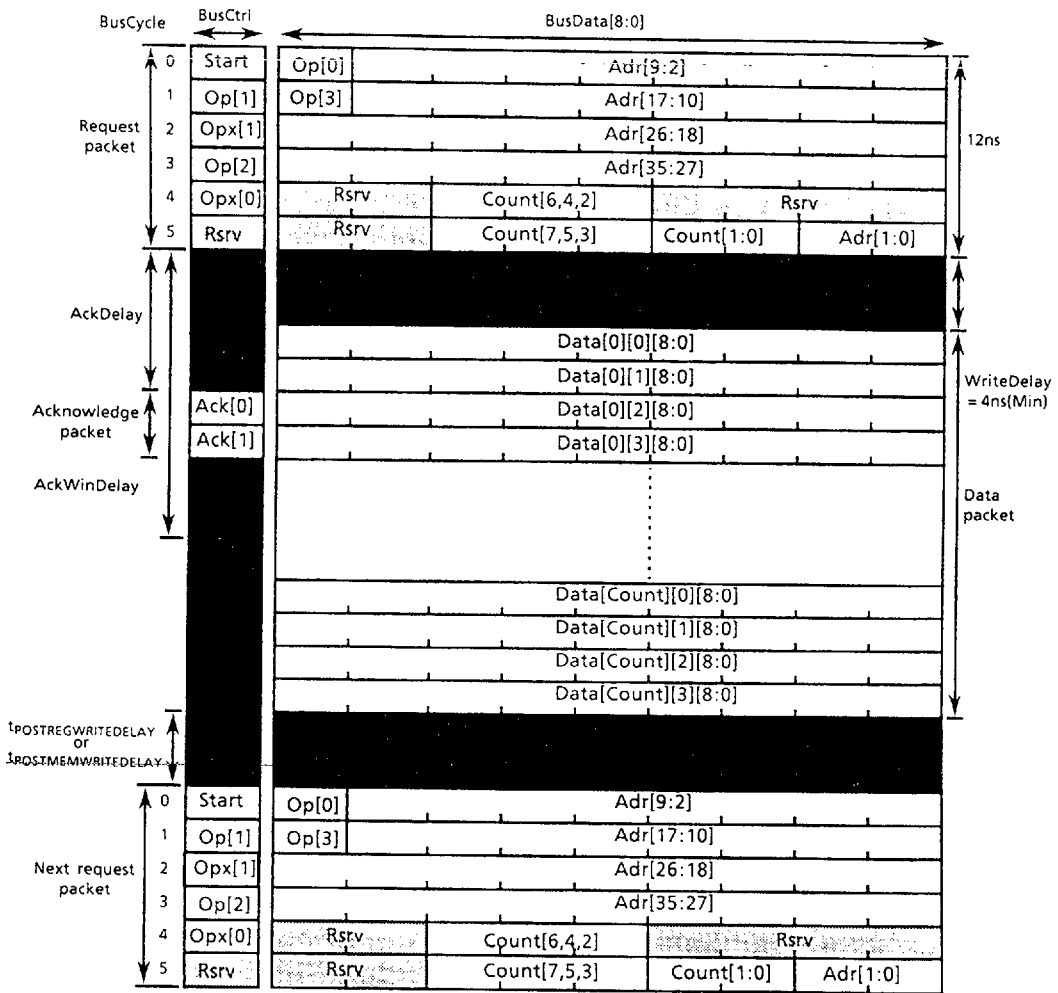
Figure 10. Write Operation for Memory or Register Address Space (Ack packet = Okay)
