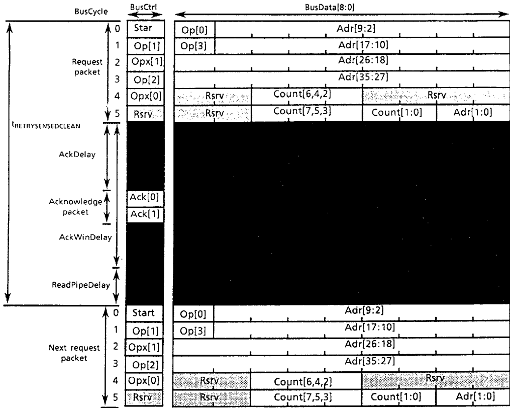
Figure 9. Read Operation for Memory or Register Address Space (Ack packet = Nack or Nonexistent)
