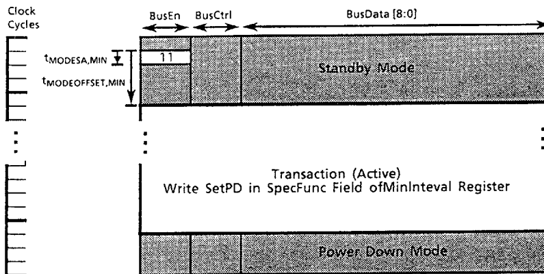
Figure 27. Active Mode to Power Down Mode Transition
