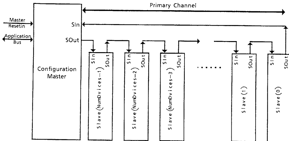
Figure 32. Shows a Rambus System with a Single Configuration Wafer Device a Single Primary Channel
