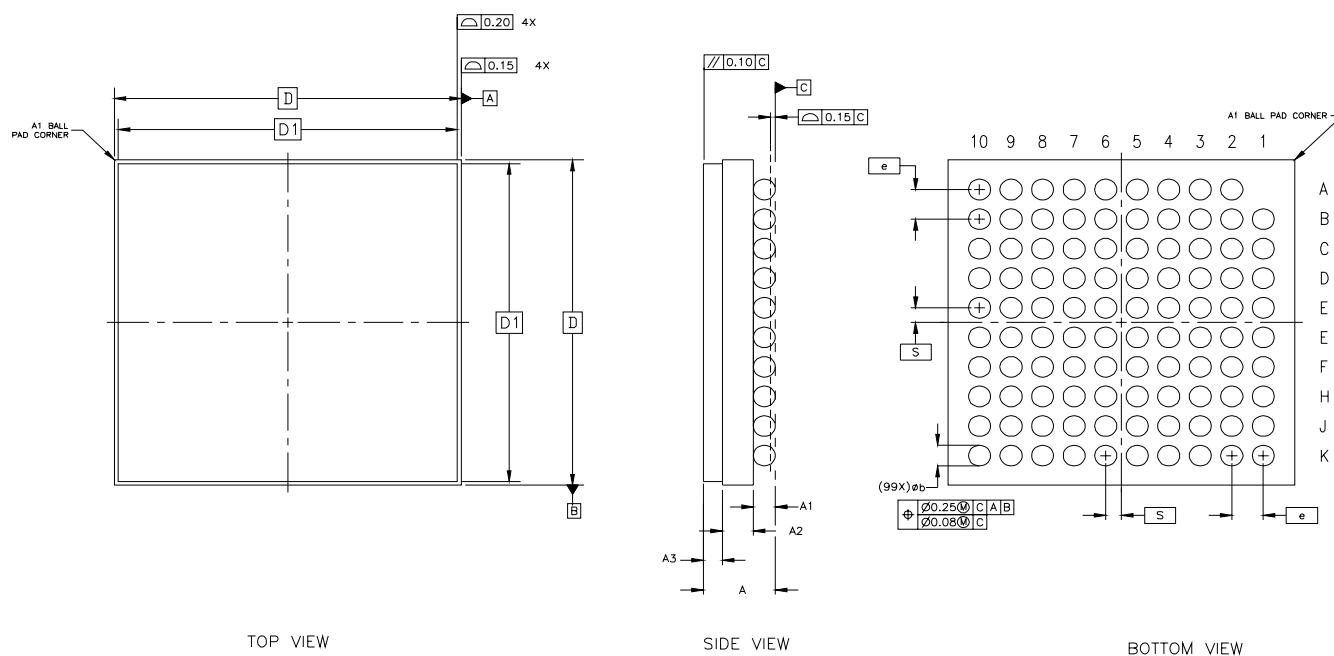
Figure 16. 99-Ball Ceramic Ball Grid Array (CBGA)
