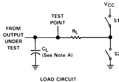
LOAD CIRCUIT
