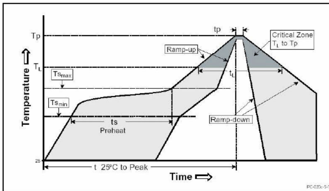
Figure 8. Reflow Profile
