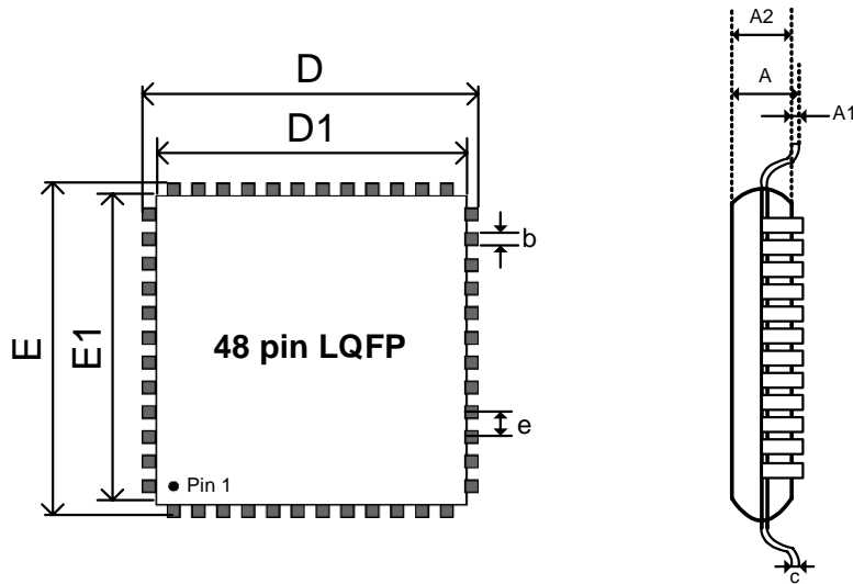
Figure 7. 48-Pin LQFP Package Outline and Package Dimensions
