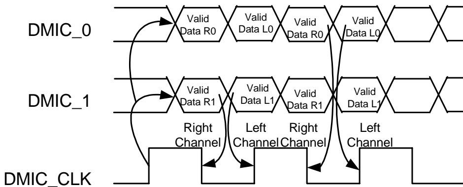
Figure 3. Quad Digital Microphone Configuration
