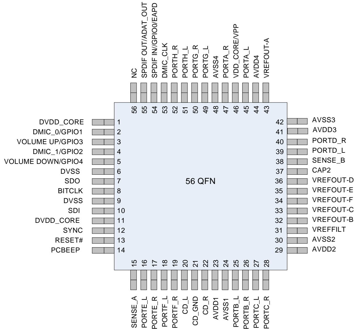
Figure 5. 56-Pad QFN Pinout
