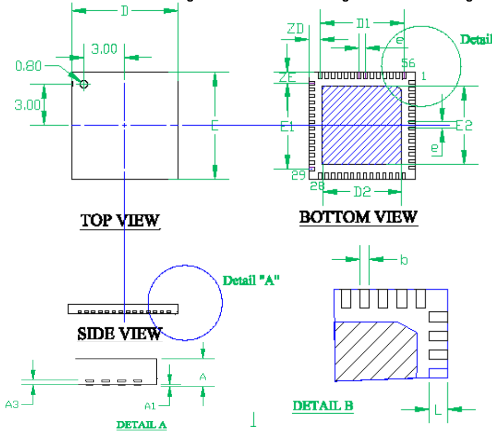
Figure 6. 56-Pad QFN Package Outline and Package Dimensions
