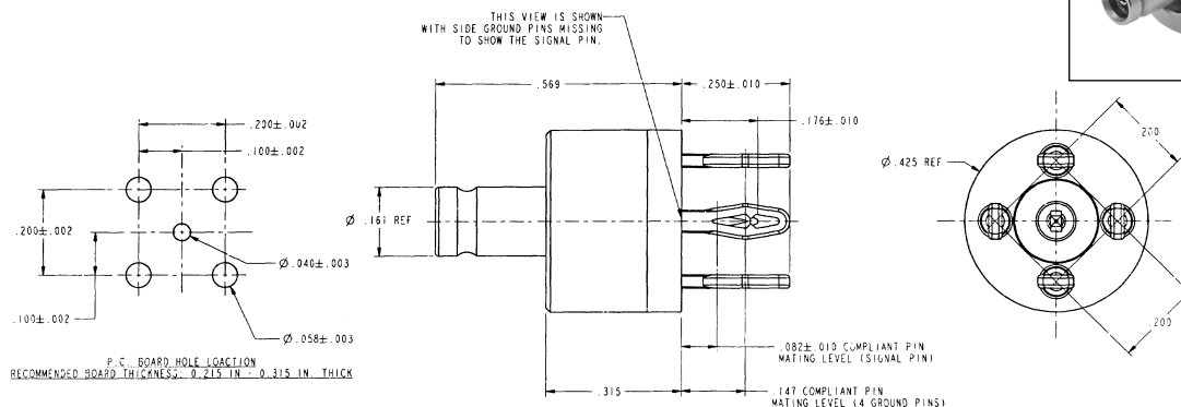
PCB Press Fit Jack 102-909-D100
