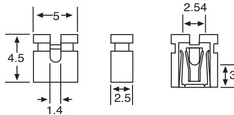
Part Number - MJ2S Description - Open Top
