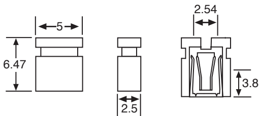
Part Number - MJ2MH Description - Closed Top
