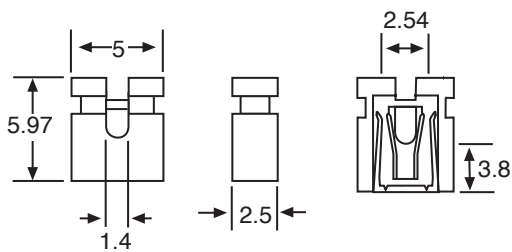
Part Number - MJ2MS Description - Open Top
