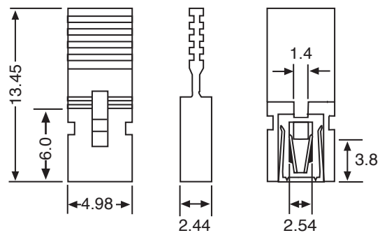
Part Number - MJ2UH Description - Open Top
