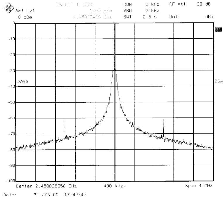
Figure 9. TX spectrum Pout = 1.4 dBm (corrected for cable attenuation: 2 dB) Spurious signal suppression > 60 dBc (typical) PLL loop filter values optimized for settling time < 150 μs
