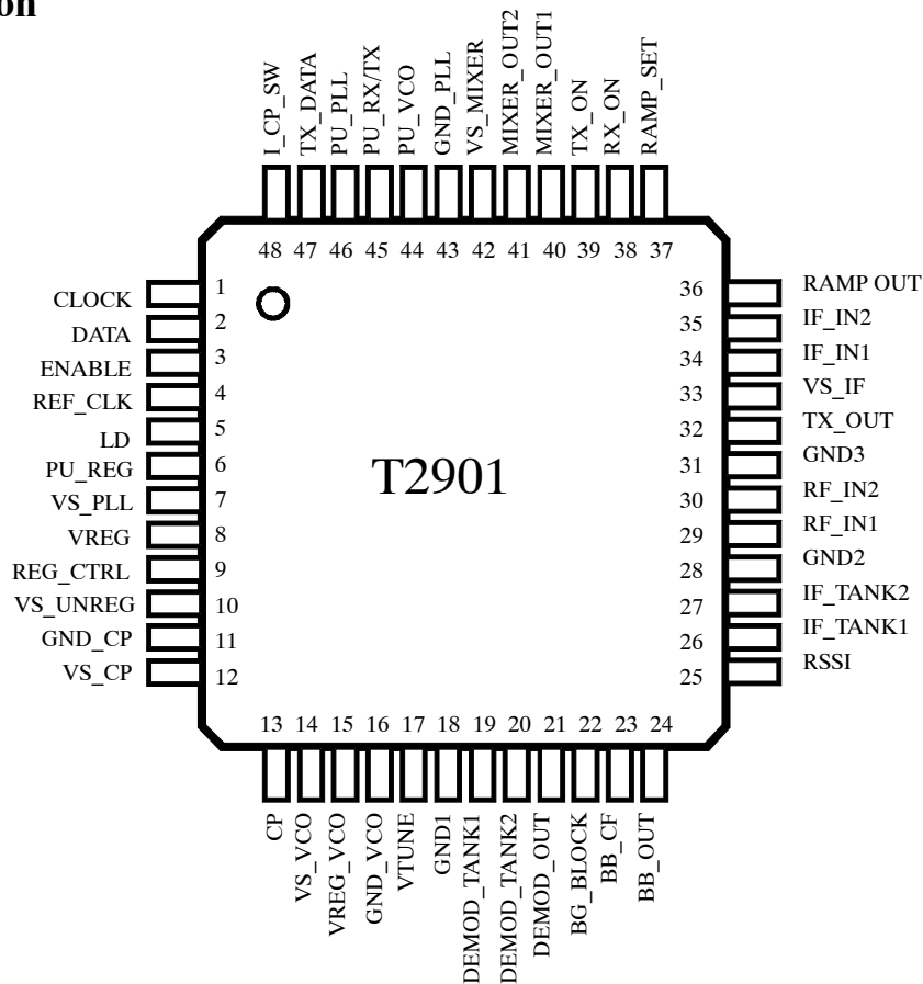
Figure 2. Pinning
