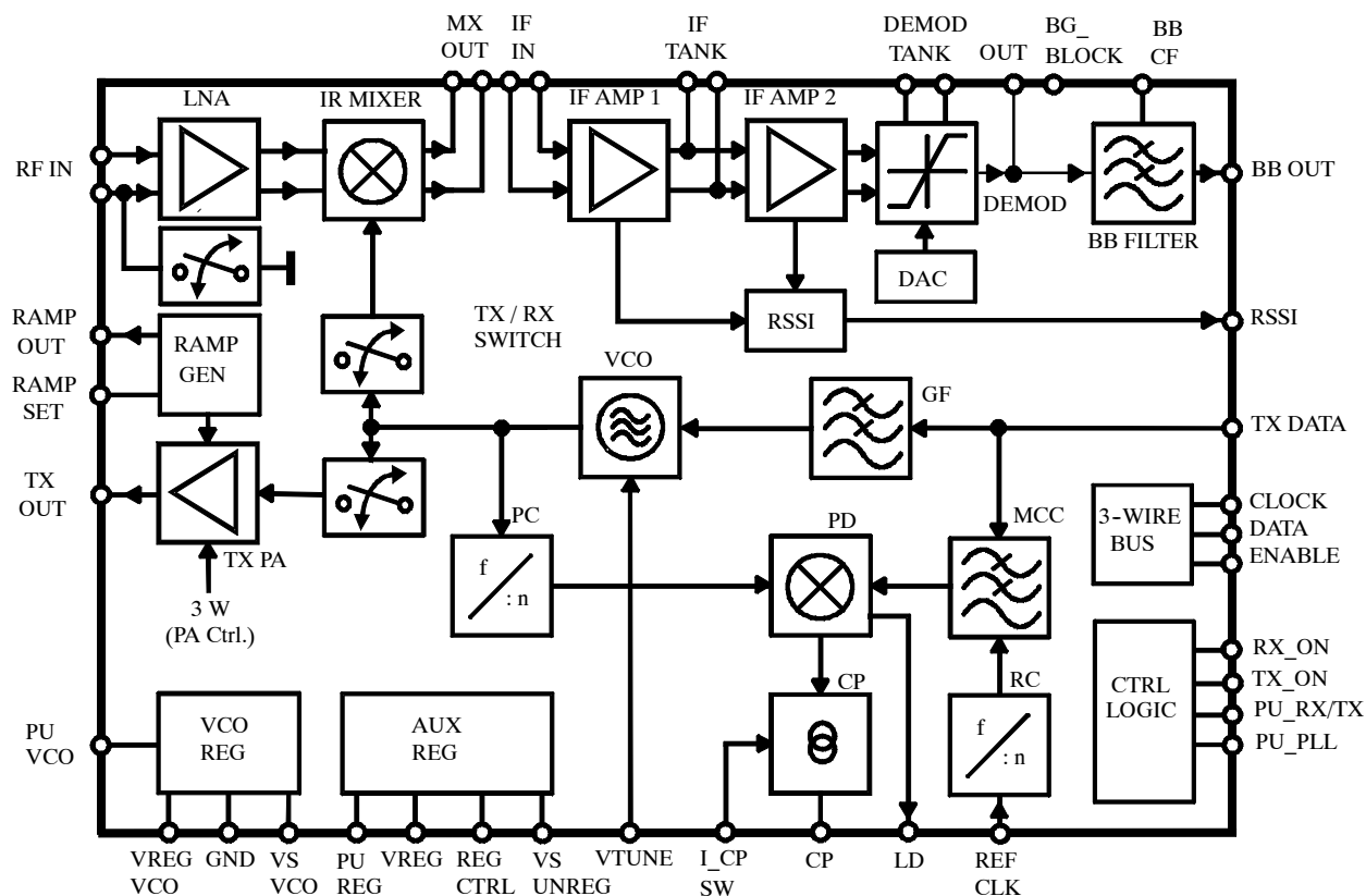
Figure 1. Block diagram
