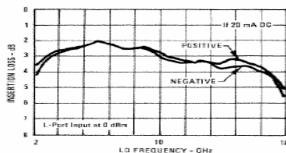
Insertion Loss with DC Driven I-Port
