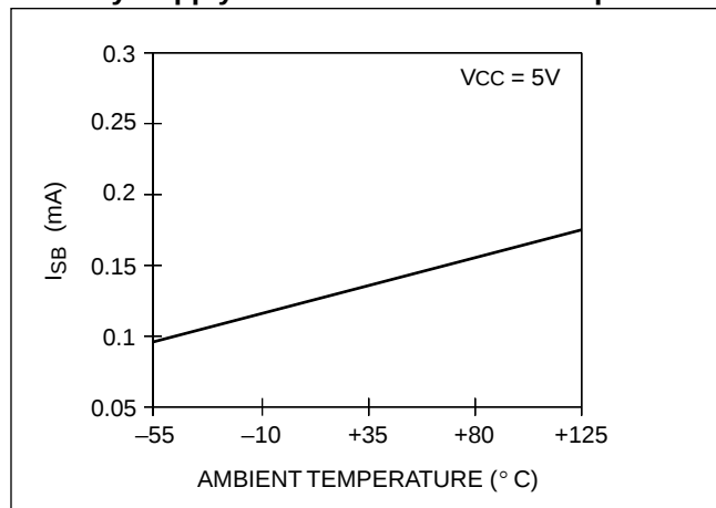
Standby Supply Current vs. Ambient Temperature
