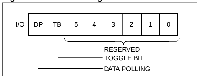
Figure 1. Status Bit Assignment
