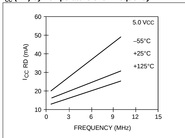
I_{CC} (RD) by Temperature over Frequency
