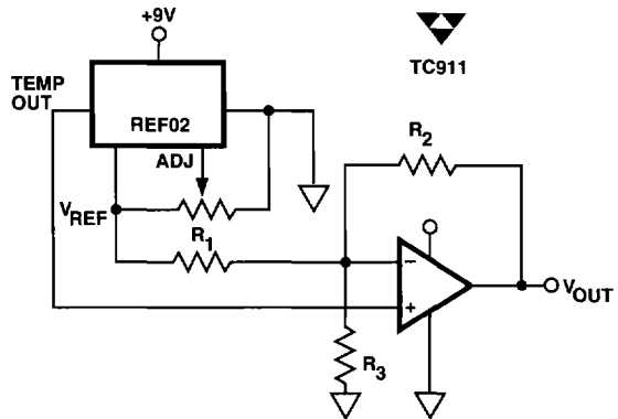
Thermometer Circuit
