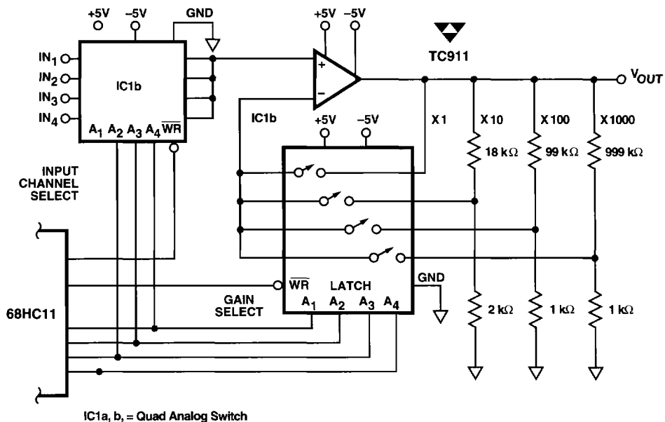
Programmable Gain Amplifier With Input Multiplexer
