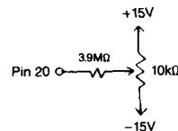
OFFSET ADJUST
