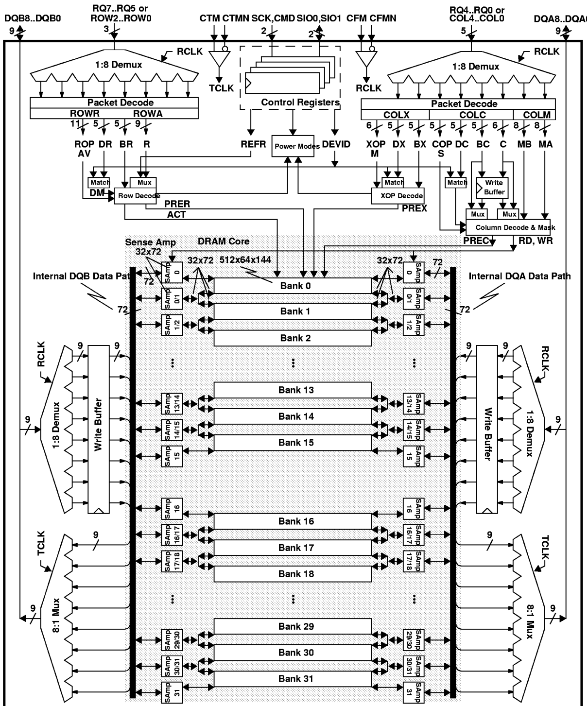
Figure 2: 128/144 Mbit Direct RDRAM Block Diagram
