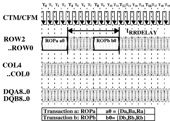
Figure 6: ROW-to-ROW Packet Interaction- Timing
