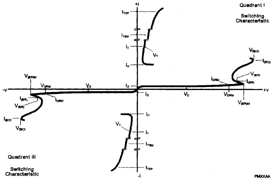
Figure 1. VOLTAGE-CURRENT CHARACTERISTICS
