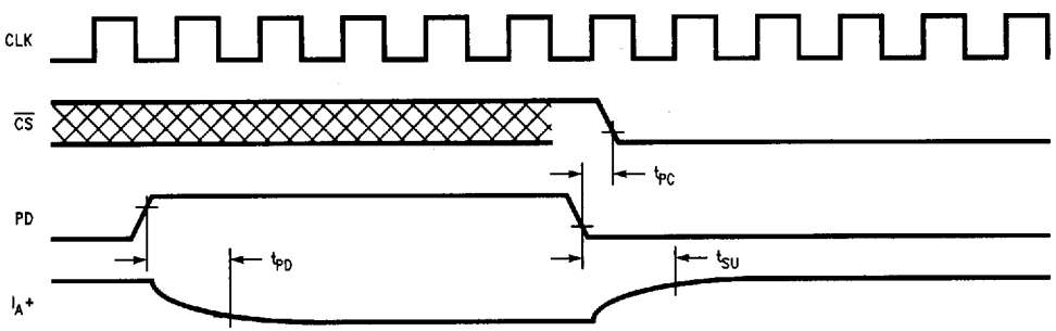
FIGURE 5. Hardware Power Up/Down Sequence
