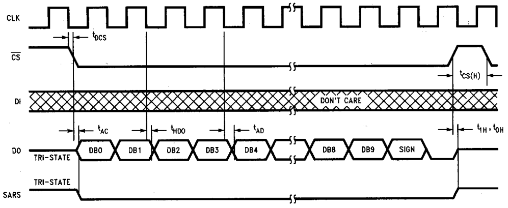
FIGURE 4. Delayed DO Timing
