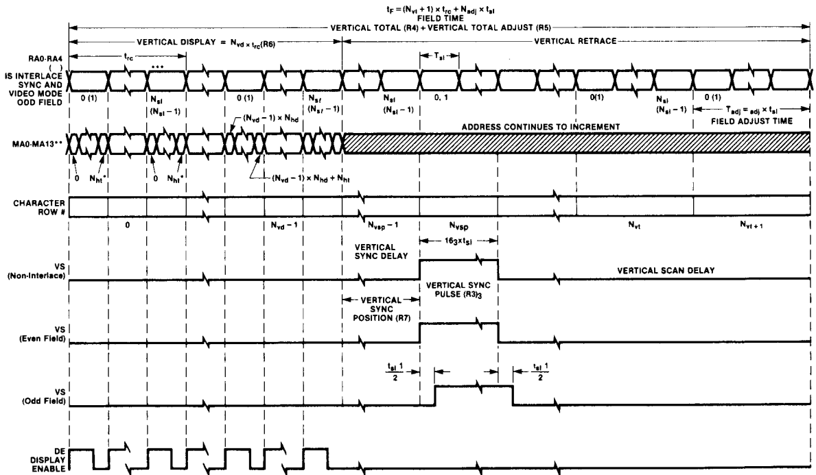
Figure 9 CRTC Vertical Timing
