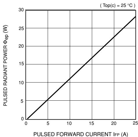
Figure 2: Radiant Power vs. Pulsed Forward Current (Typ.)
