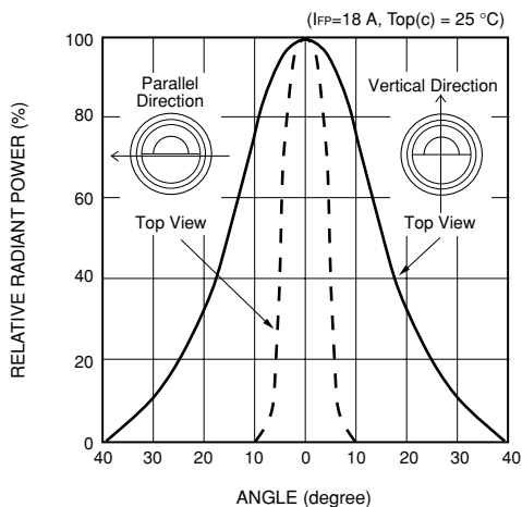
Figure 4: Directivity (Typ.)
