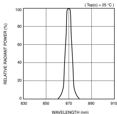
Figure 3: Emission Spectrum (Typ.)
