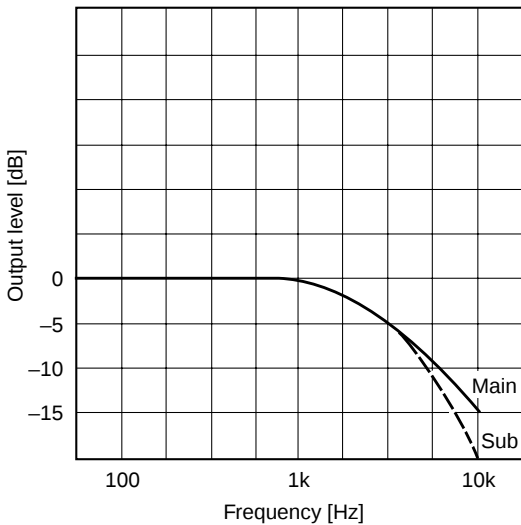
De-emphasis characteristics
