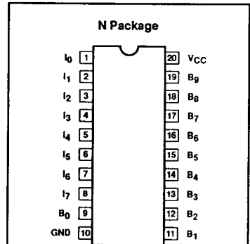
N = Plastic DIP (300mil-wide)
