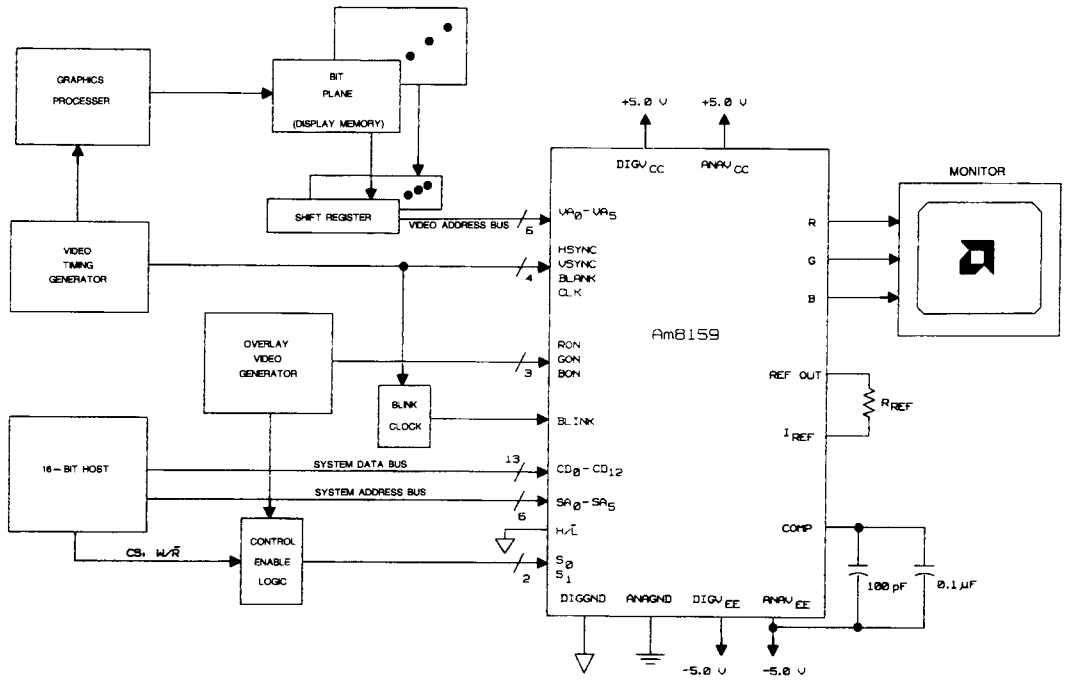
Figure 2. Typical Application Diagram
