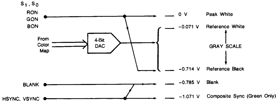
Figure 1. Am8159 DAC Output Levels
