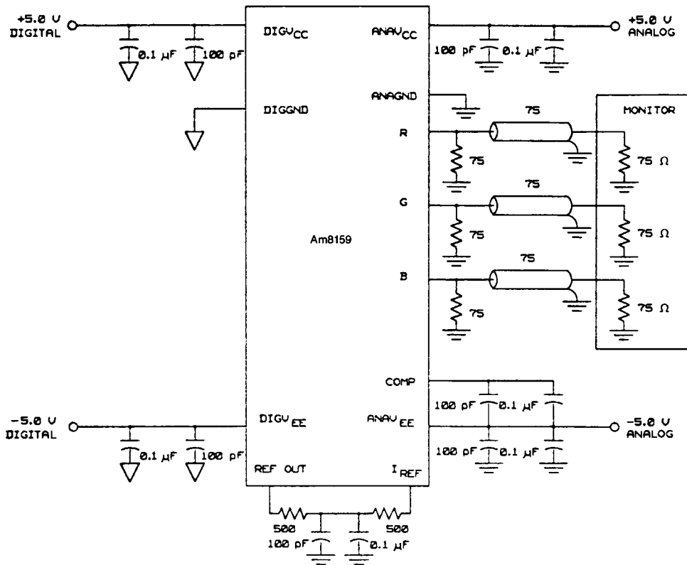
Figure 3. Typical Connection Diagram
