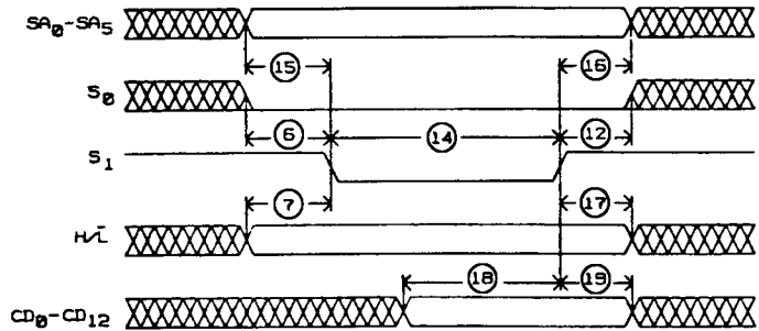
Write Timing
