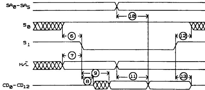
Read Timing
