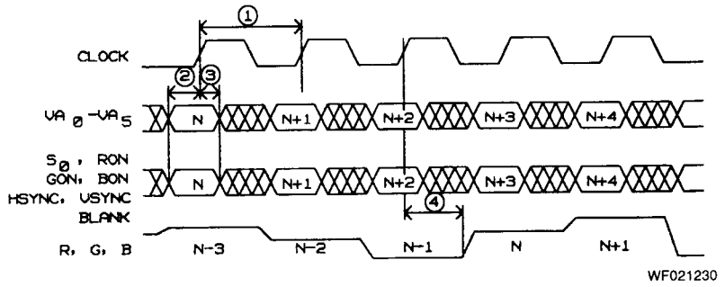
Run and Overlay Timing
