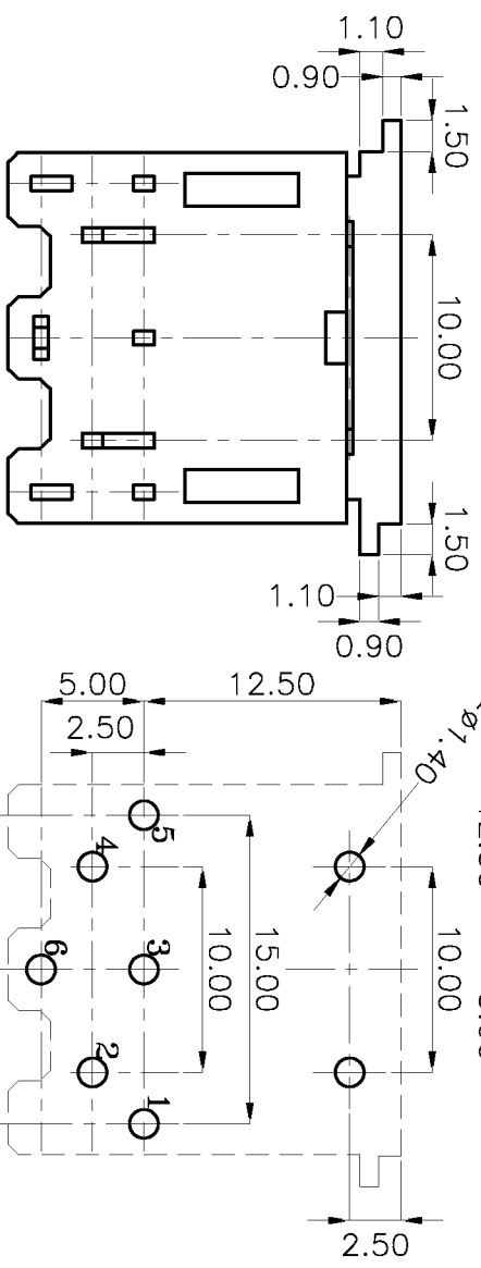
PCB LAYOUT (BOTTOM VIEW)
