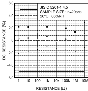
Fig.5 Resistance
