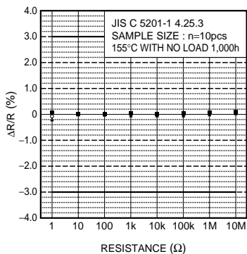
Fig.12 Endurance
