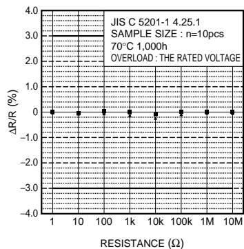
Fig.11 Endurance at 70°C
