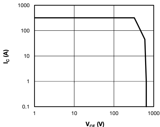
Fig. 17 - Trench IGBT Reverse BIAS SOA T_J = 175^\circ\text{C} , I_C = 320\text{ A} , R_g = 4.7\ \Omega , V_{GE} = +15\text{ V/0 V} , V_{CC} = 325\text{ V} , V_p = 650\text{ V}
