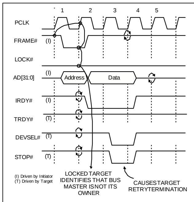
Figure 52. Access Attempt to a Locked Target
