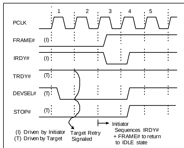
Figure 49. Target-Initiated Retry
