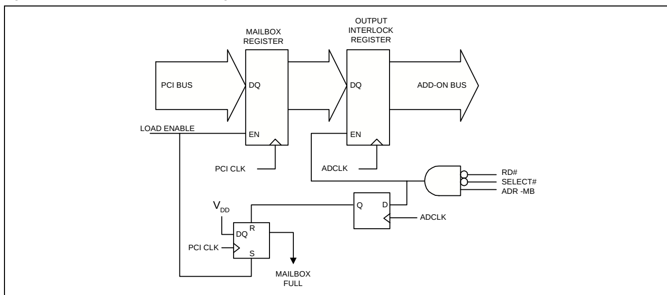
Figure 54. PCI to Add-On Mailbox Register
