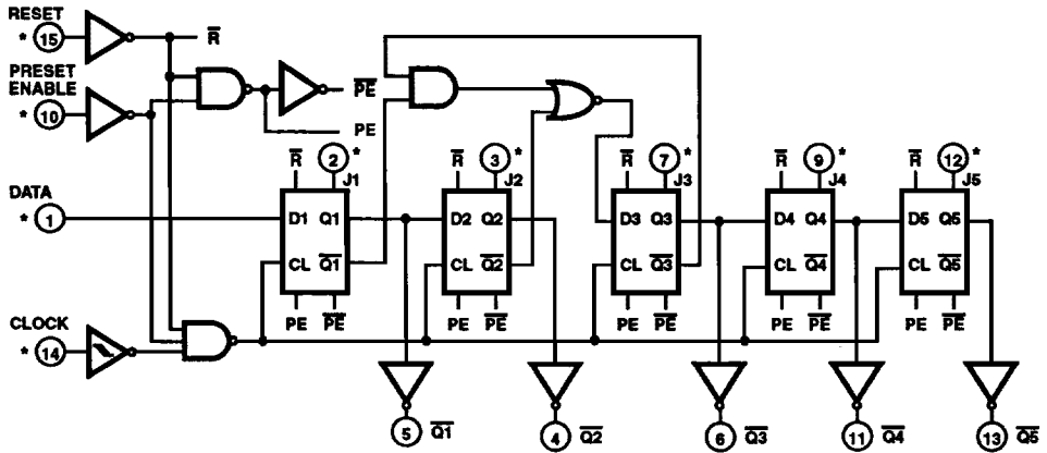
FIGURE 1. LOGIC DIAGRAM
