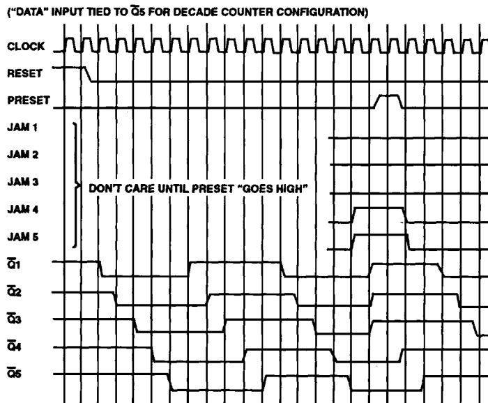
FIGURE 11. TIMING DIAGRAM
