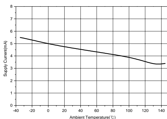
Figure 16. Supply Current vs Temperature
