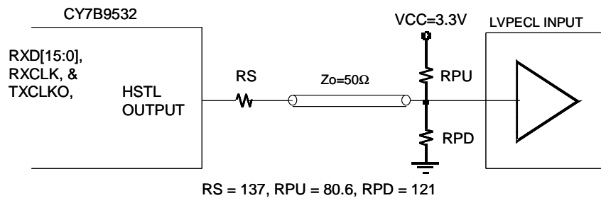
Figure 6. LVPECL Compliant Termination
