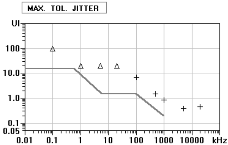
Figure 2: Jitter tolerance waveform of CY7B9532V [4]
