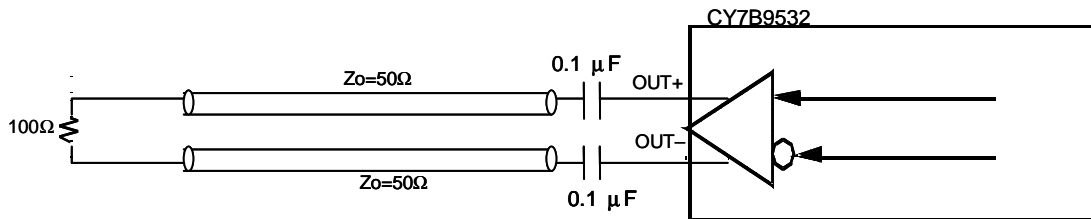
Figure 3. Serial Output Termination
