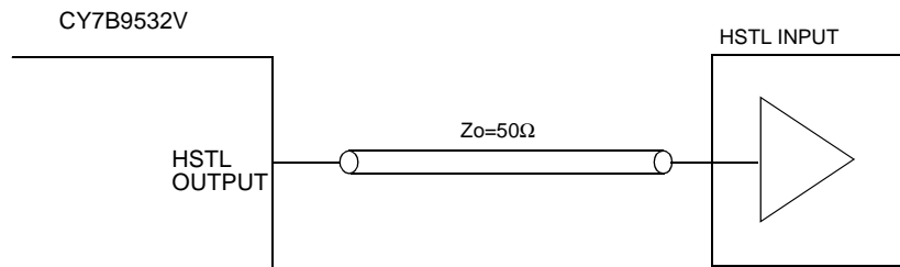
Figure 5. RXD[15:0] Termination
