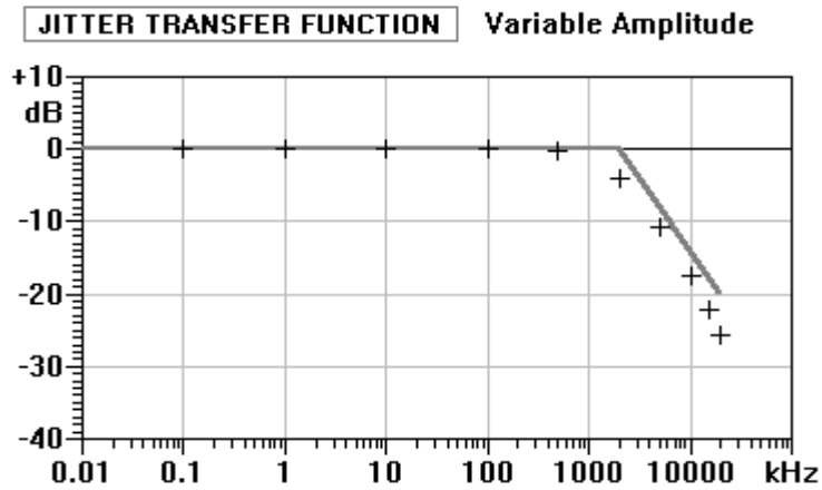
Figure 1: Jitter transfer waveform of CY7B9532V [4]
