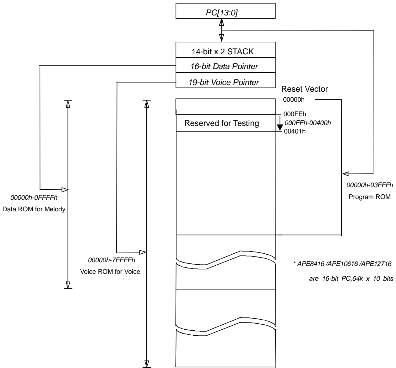
FIGURE 1 : ROM Map of APExx16 Series
