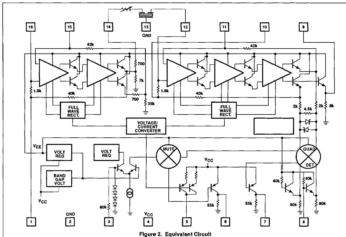
Figure 2. Equivalent Circuit
