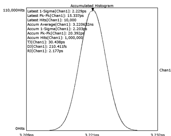
Figure 3: Period Jitter Histogram at 311.04 MHz Analog Frequency Multiplier (2x) with 155.52MHz crystal
