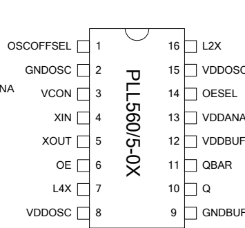
4X AFM Package Pin Out
