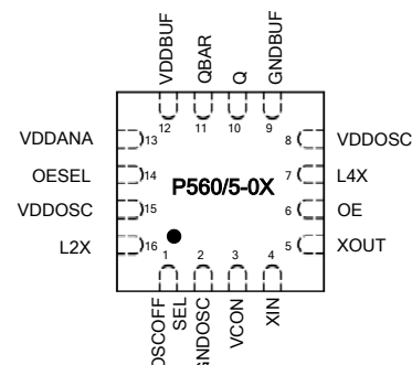
4X AFM Package Pin Out
