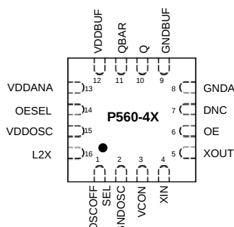
2X AFM Package Pin Out
